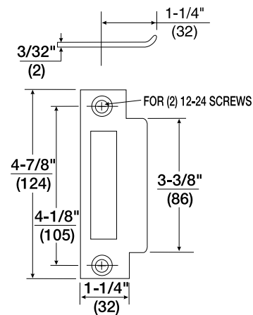
2815 Curved Lip Strike (1-1/4"/32mm standard)
