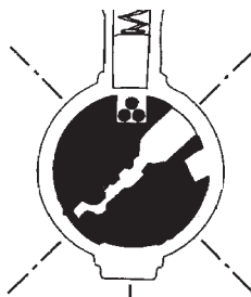
As change key rotates, construction balls fall into hole in the side of plug
