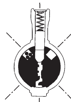
Construction key inserted after balls are trapped. Top pin now extends into plug chamber. Construction key will not rotate
