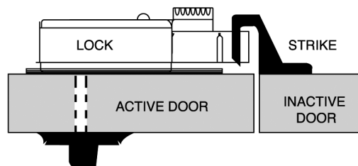
TYPE 9 Part# 114006
