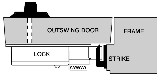
TYPE 2 Part# 114004
