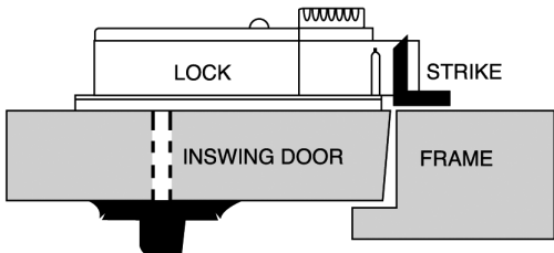
TYPE 3 Part# 114005
