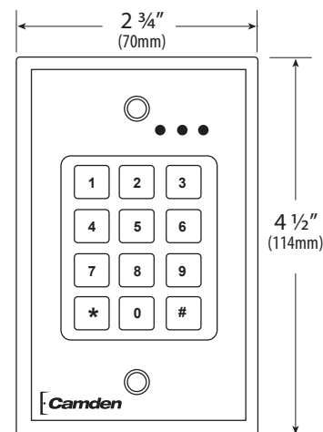
FRONT CM-120
