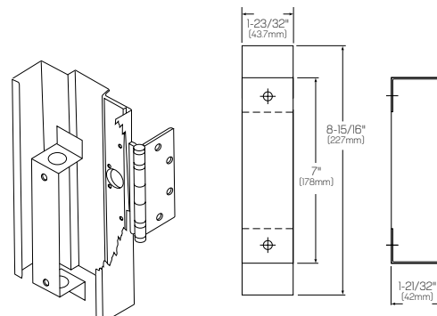
Junction Box Top View
