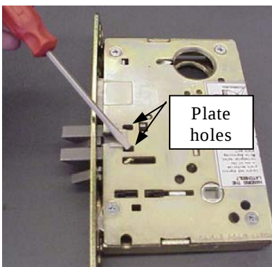
Step 1. Locate Plate in ONE of the Plate Holes.
