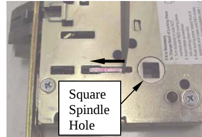
Step 2. Move Locking Piece away from Square Spindle Hole.
