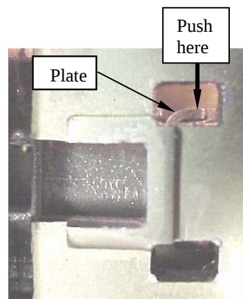
Step 2. Exploded view of Plate where screw driver presses.
