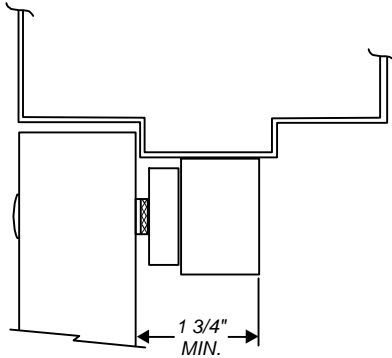
NORMAL MOUNTING
