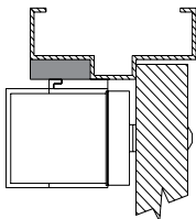
Fig. 1B With Filler Plate Refer to Filler Plates and Angle Bracket datasheet for proper filler plate specification.
