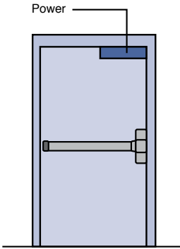
Door Movement Trigger by Latching Exit Device Rim Mount, Mortise, or Vertical Rod
